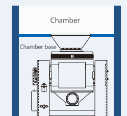
Connect shaker and chamber through head expander
